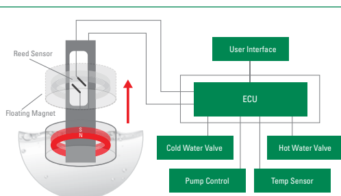
Figure 8-Float sensor detecting water level in a dishwasher
