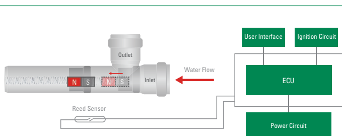
Figure 9-Flow detection in a tankless water heater
