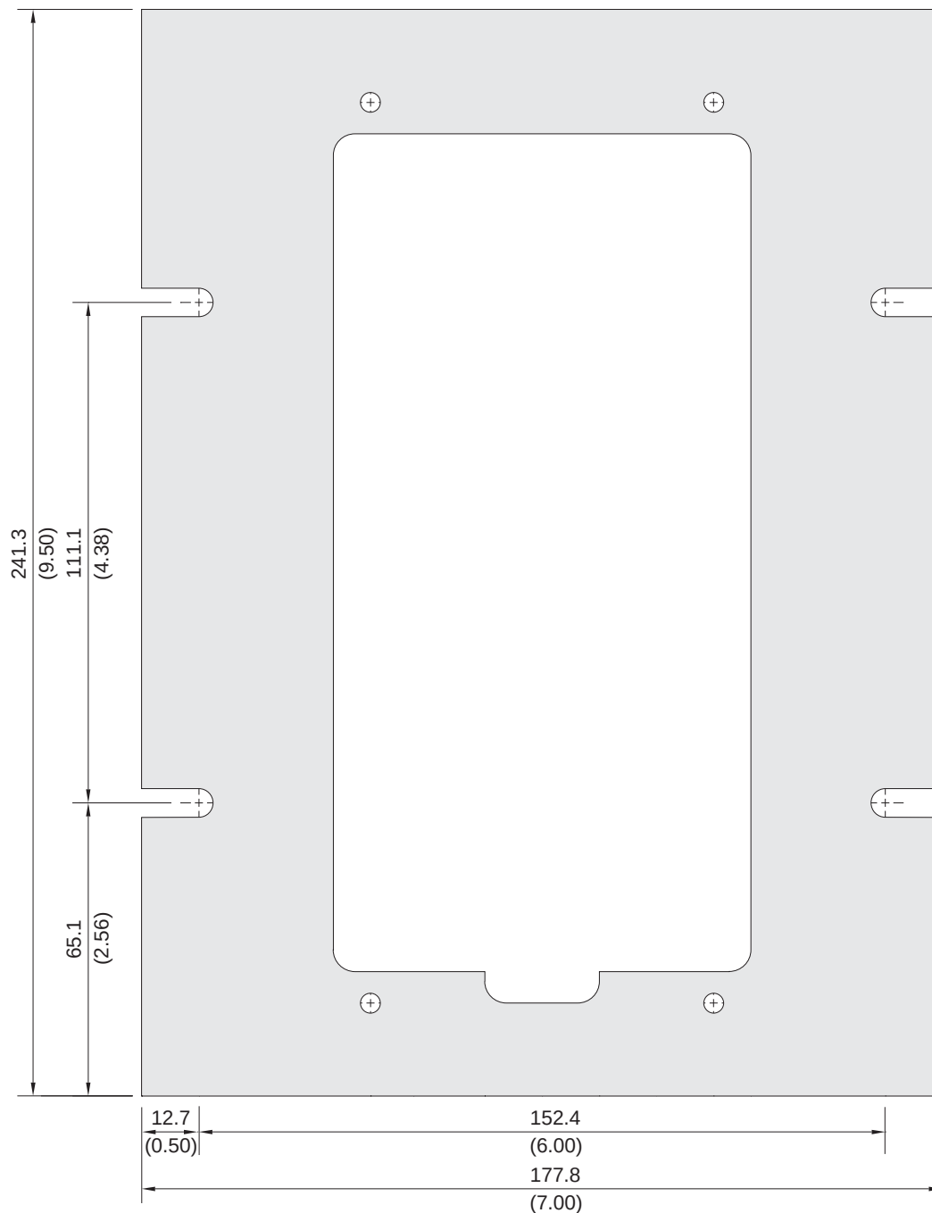
FRONT VIEW
