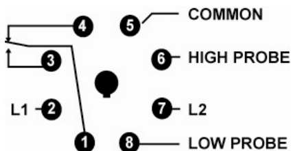
Figure 1: Pin-Out Diagram
