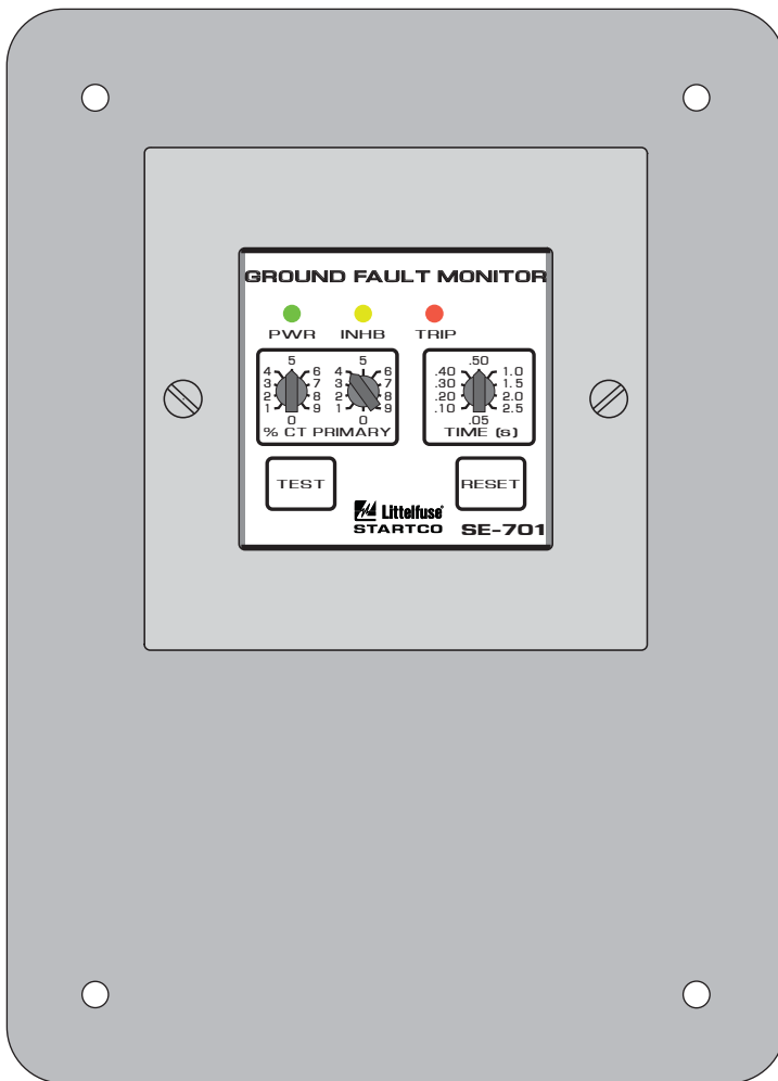
FRONT VIEW
